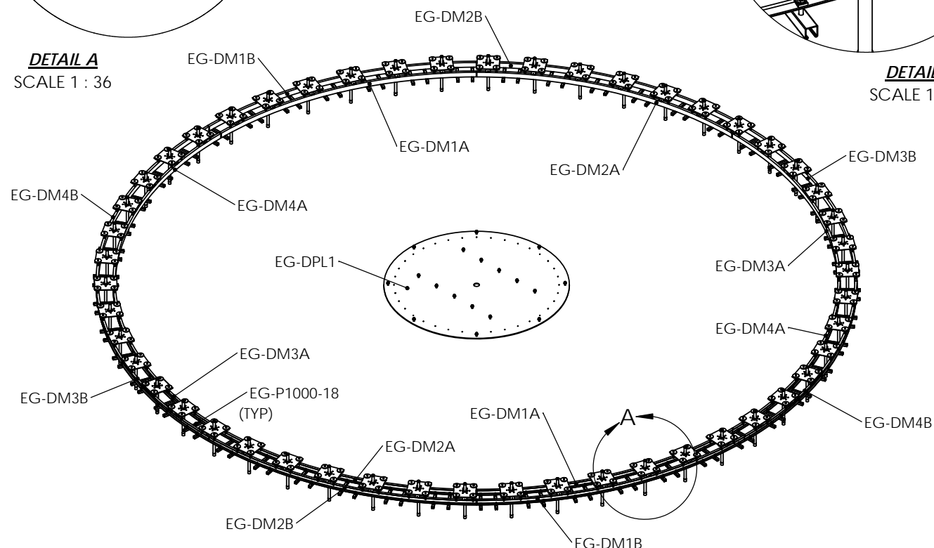
DOPPLER MOUNT ASSEMBLY SCALE 1 : 96
