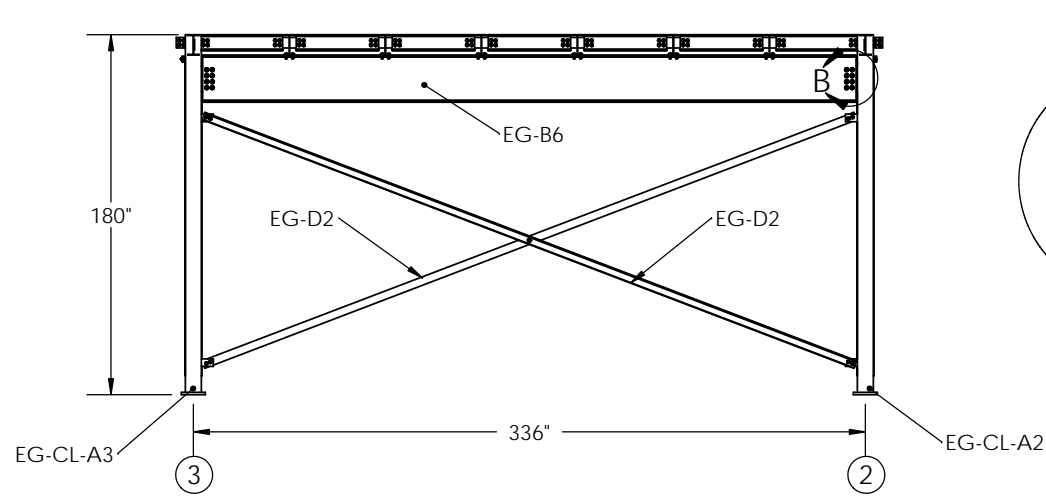
COLUMN BRACING @ LINE A SCALE = 1:96
