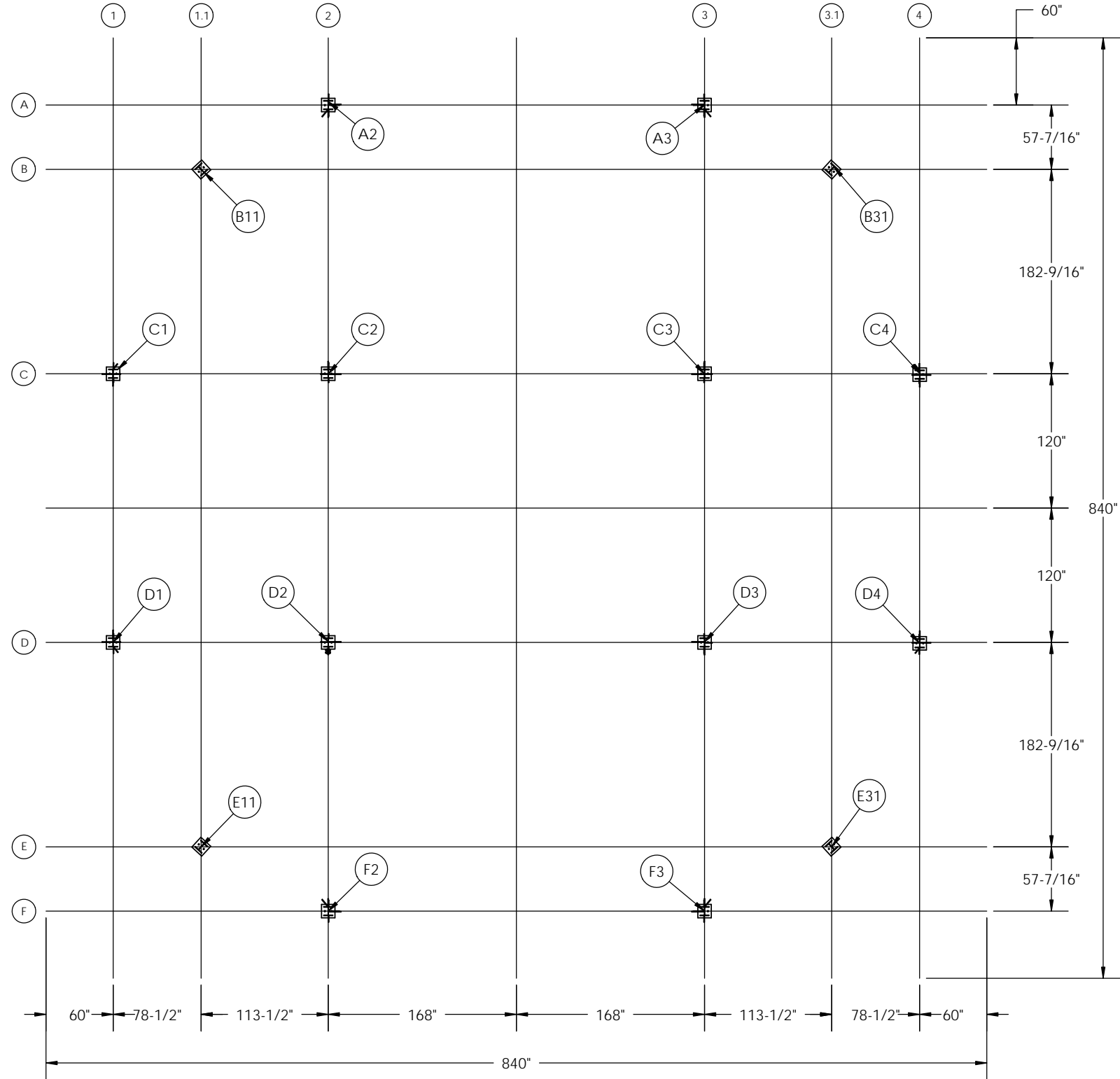
PLAN VIEW - FOUNDATION LAYOUT SCALE = 1 : 120
