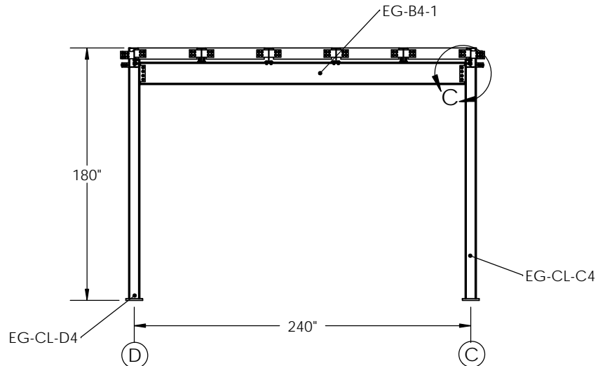
COLUMN BRACING @ LINE 4 SCALE = 1:96
