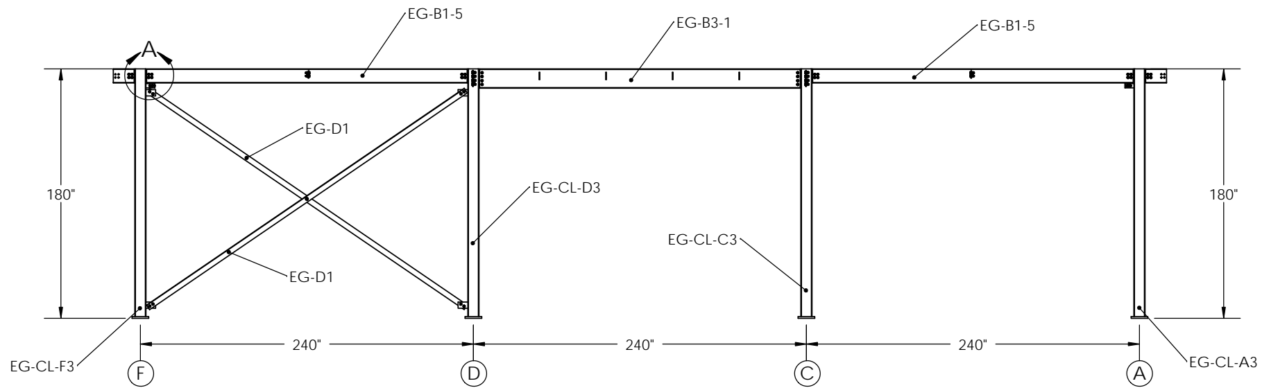
COLUMN BRACING @ LINE 3 SCALE 1 : 96
