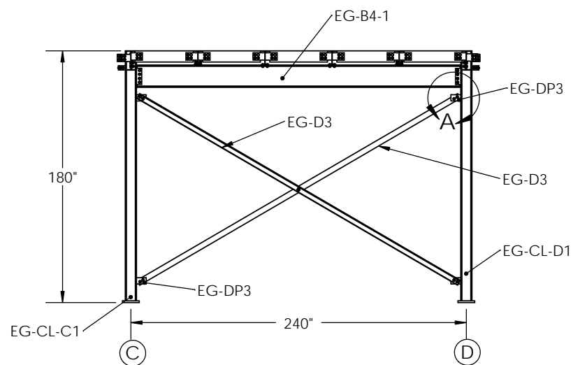
COLUMN BRACING @ LINE 1 SCALE = 1:96
