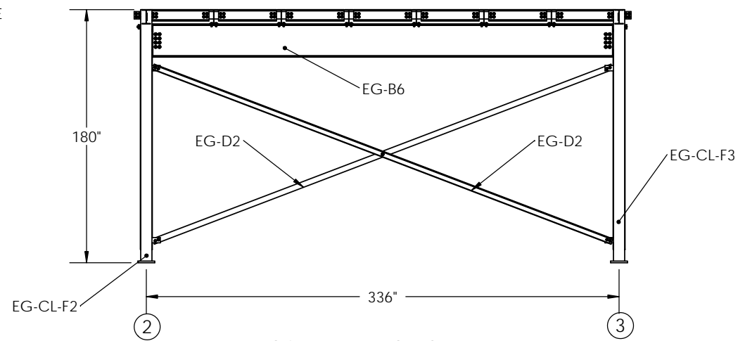
COLUMN BRACING @ LINE F SCALE = 1:96
