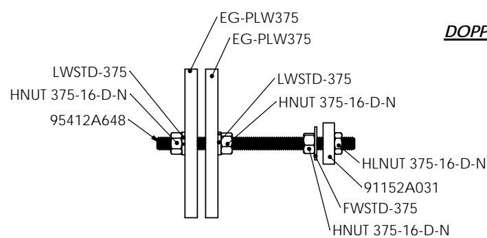
PLATE WASHER ASSEMBLY MK. PLW375 (ASSY)
